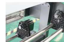
External power supply, intelligent rolling system.
